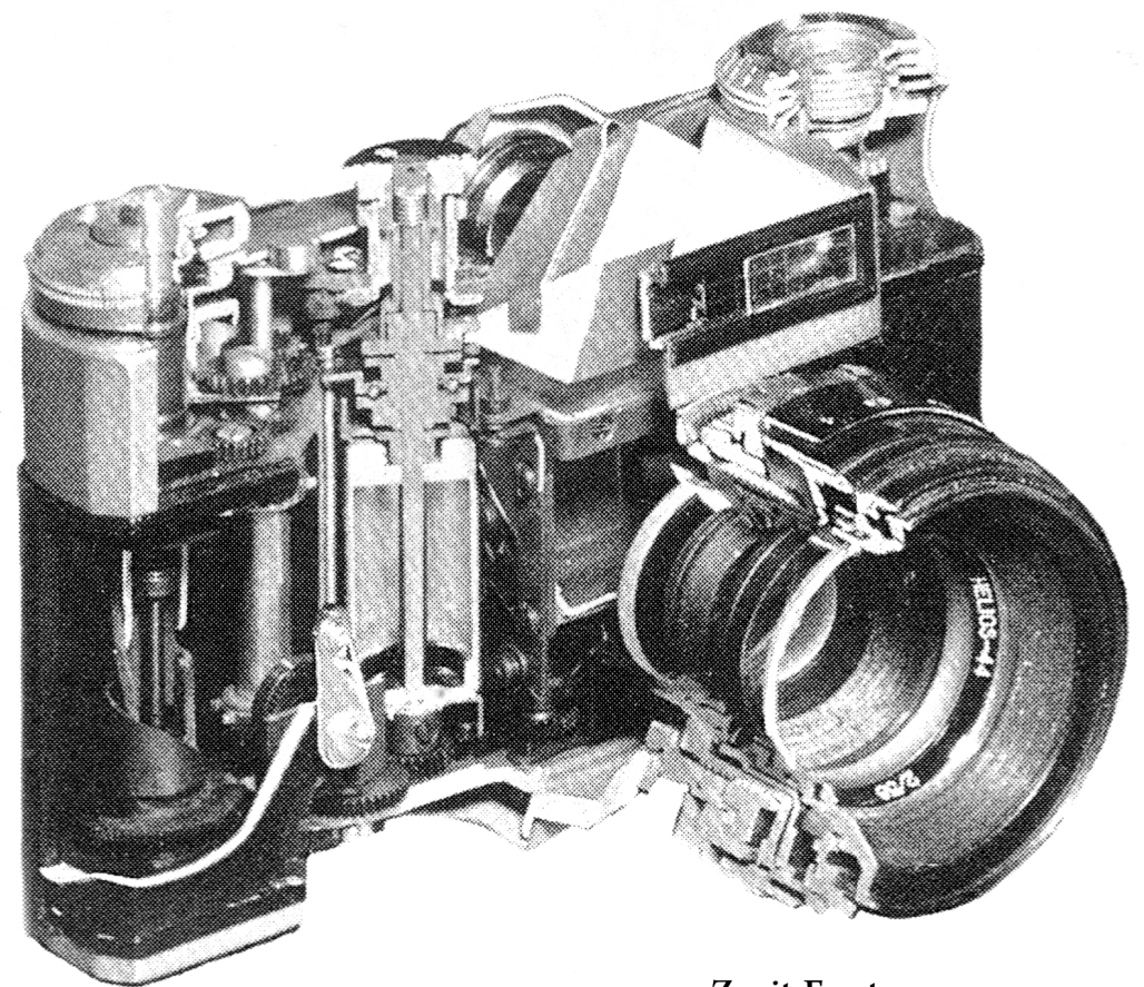
Zenit-E cutaway
